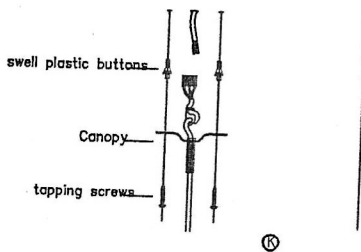
K. Install the swell plastic buttons into the ceiling. Use the tapping screws to fix the bracket into the ceiling. L. Connect the power wire to the terminal block. M. Fix the canopy to the bracket by screws.
