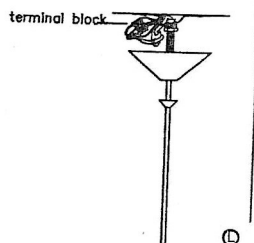
K. Install the swell plastic buttons into the ceiling. Use the tapping screws to fix the bracket into the ceiling. L. Connect the power wire to the terminal block. M. Fix the canopy to the bracket by screws.
