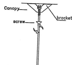
K. Install the swell plastic buttons into the ceiling. Use the tapping screws to fix the bracket into the ceiling. L. Connect the power wire to the terminal block. M. Fix the canopy to the bracket by screws.
